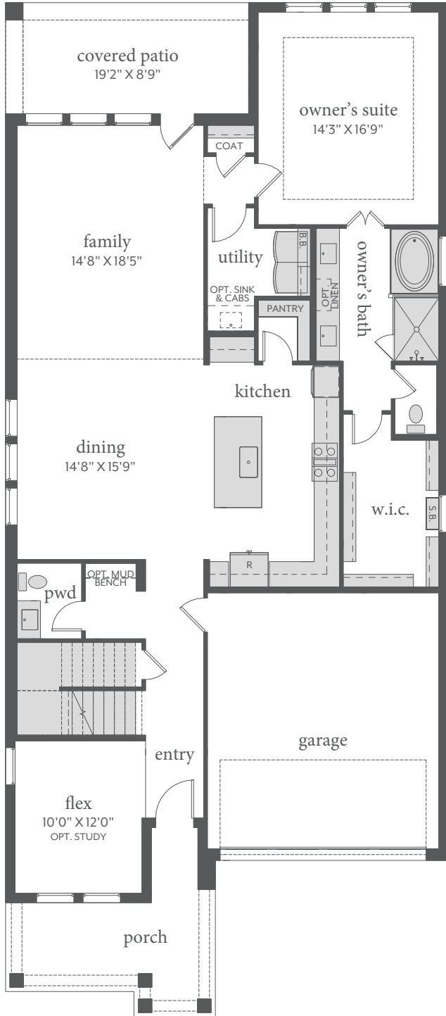
FIRST FLOOR - ELEVATION A*
