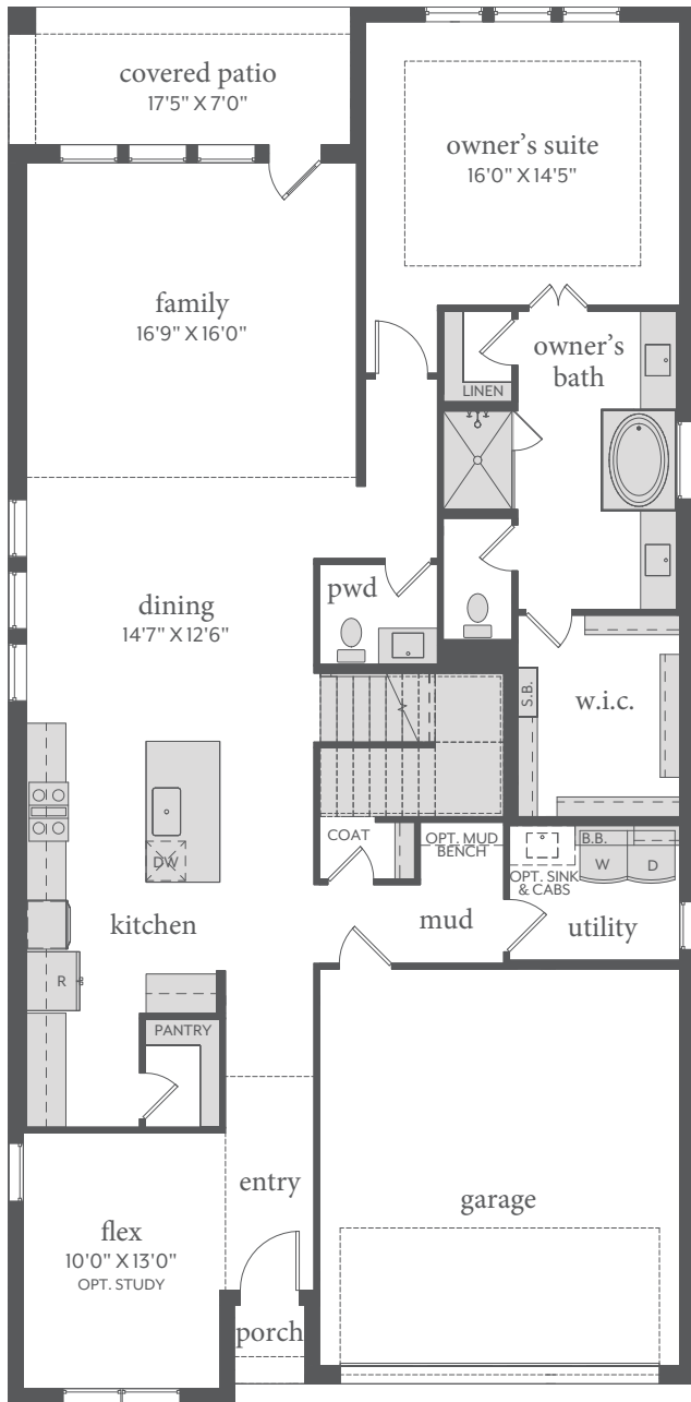
FIRST FLOOR - ELEVATION A*
