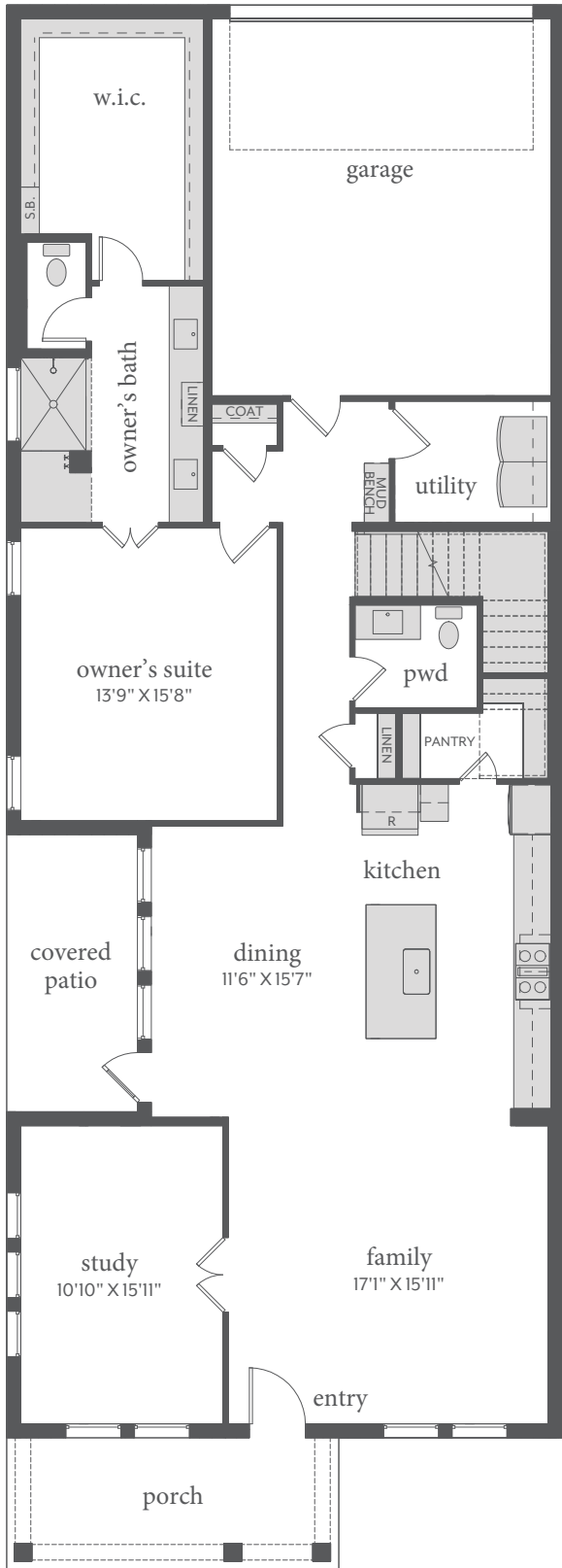
FIRST FLOOR - ELEVATION A*
